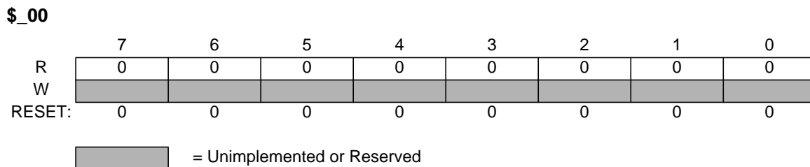
Figure 3-1 Reserved Register (ATDCTL0)
